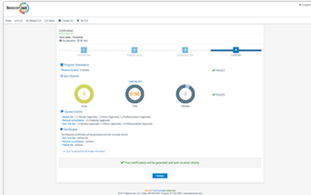
CE Workflow
